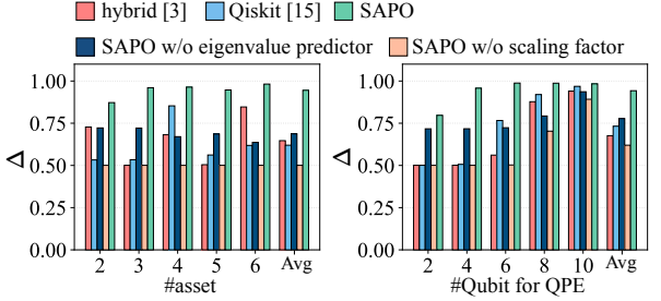
(a) Accuracy under 5-qubit QPE across different number of assets. (b) Accuracy under 5-asset problem across different number of qubits.
