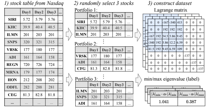
(a) Constructing the dataset for 3-assets problem using Nasdaq market data. The values in the Lagrange matrix need to multiply 10^{-5} .
